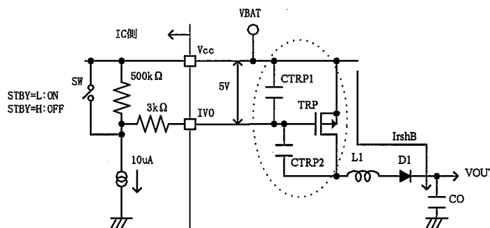
Figure 8. Step-up DC/DC basic configuration diagram of this IC
