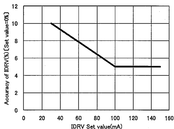
Figure 11. Accuracy of IDRv vs Settings of IDRv
