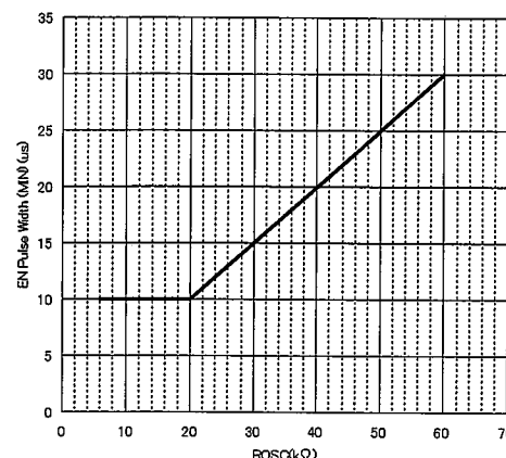
Figure 5. Pulse width (MIN) vs. RO SC
