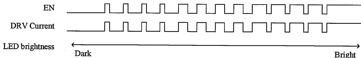
Figure 4. EN pulse vs. IDRV
