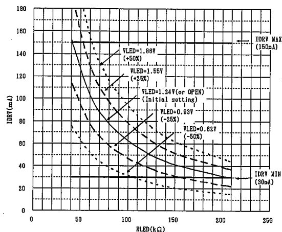
Figure 3. RLED vs. IDRV
