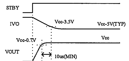
Figure 9. STBY→VOUT timing diagram
