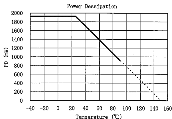
Figure 10. Power Dissipation
