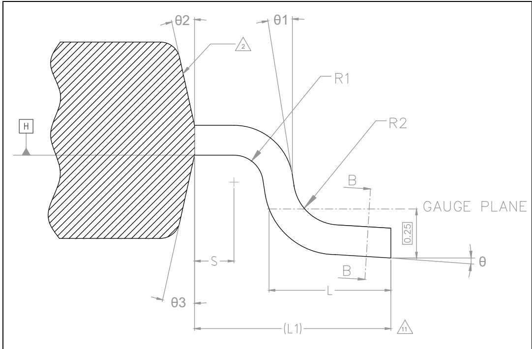
Figure 50. eTQFP144 section A-A
