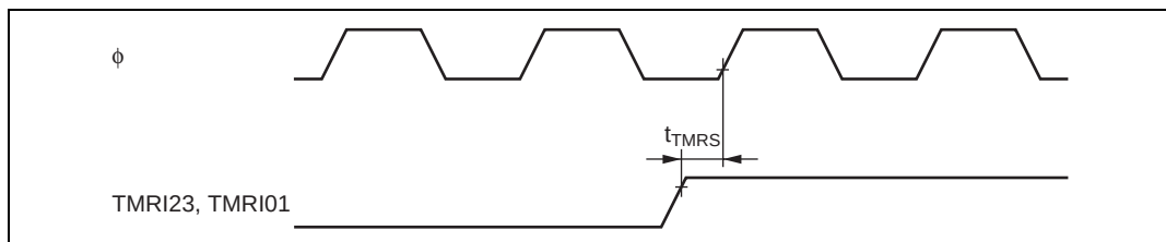
Figure 24.17 8-Bit Timer Reset Input Timing
