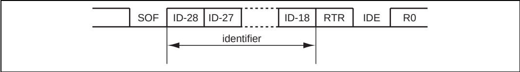
Figure 15.3 Standard Format
