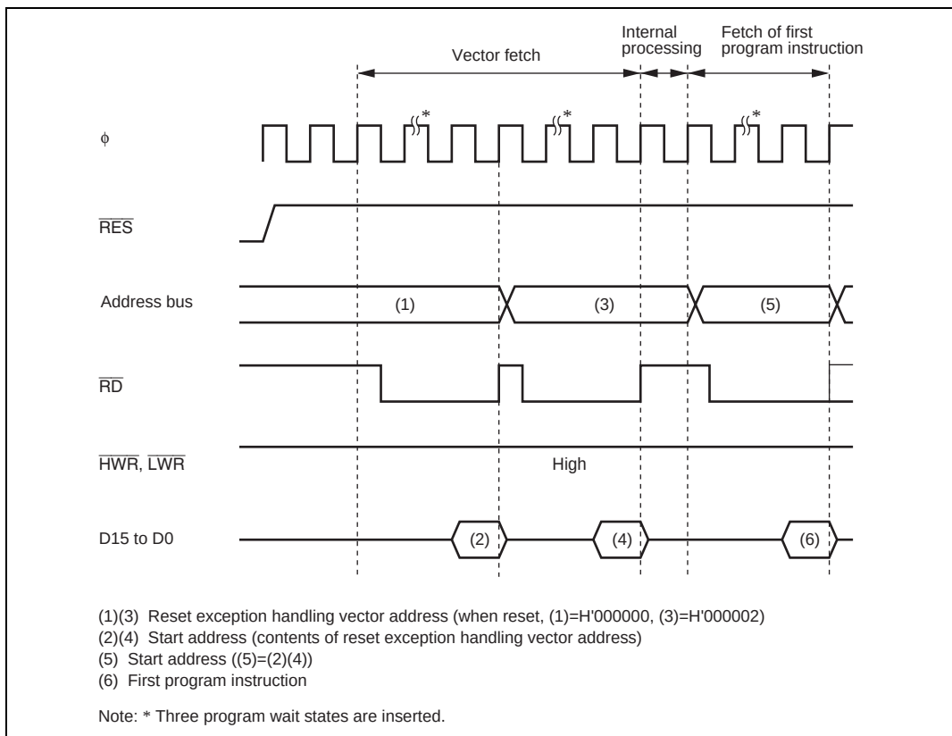
Figure 4.2 Reset Sequence
