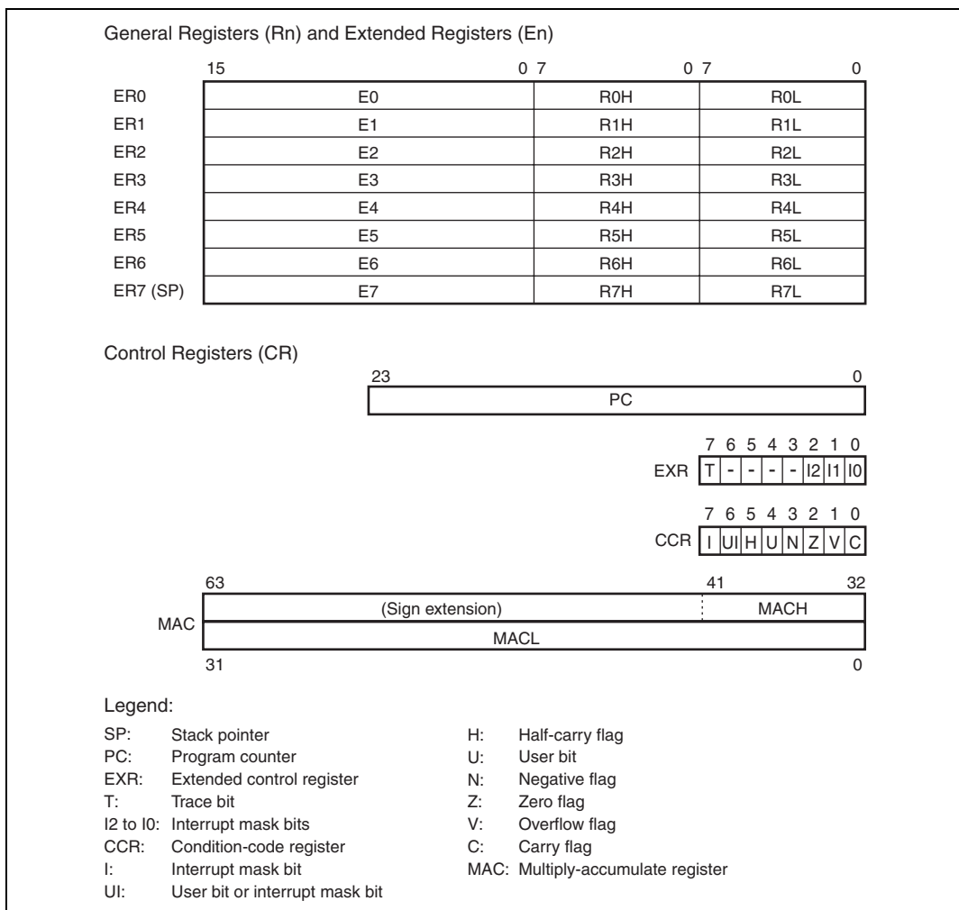
Figure 2.6 CPU Registers
