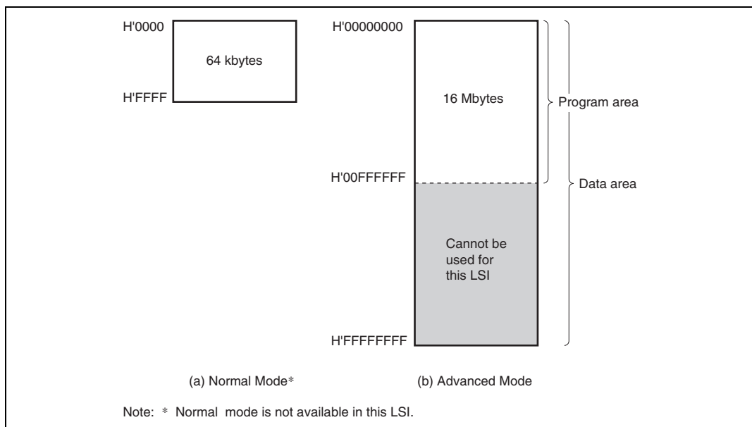
Figure 2.5 Memory Map
