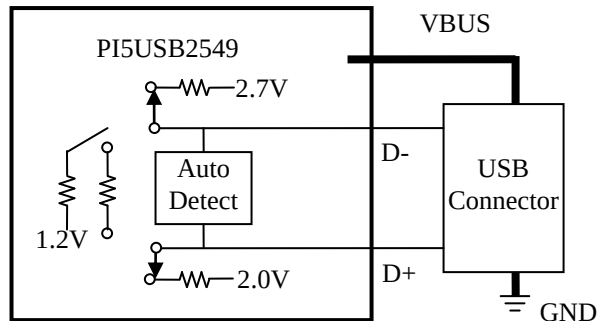
Figure 3a, Divider-1A Charging Scheme (with MODE_SEL="LOW")
