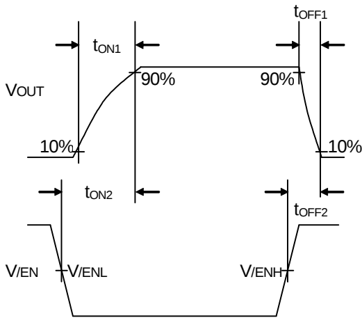
Figure 3. Timing Diagram(BD2069FJ-M)
