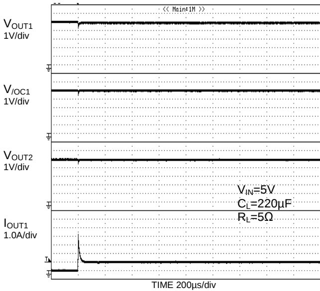
Figure 33. Inrush Current
