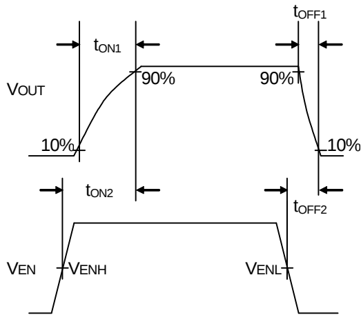
Figure 2. Timing Diagram(BD2068FJ-M)
