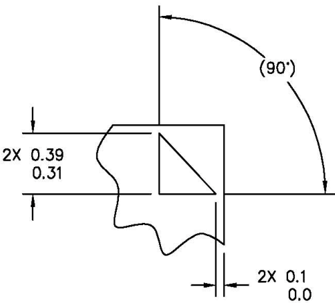
DETAIL T
