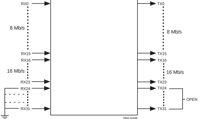
Figure 5. Split Mode
