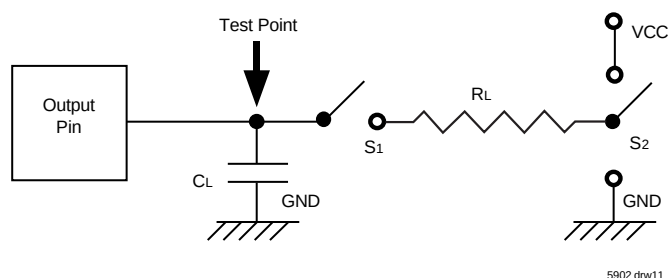
Figure 9. Output Load
