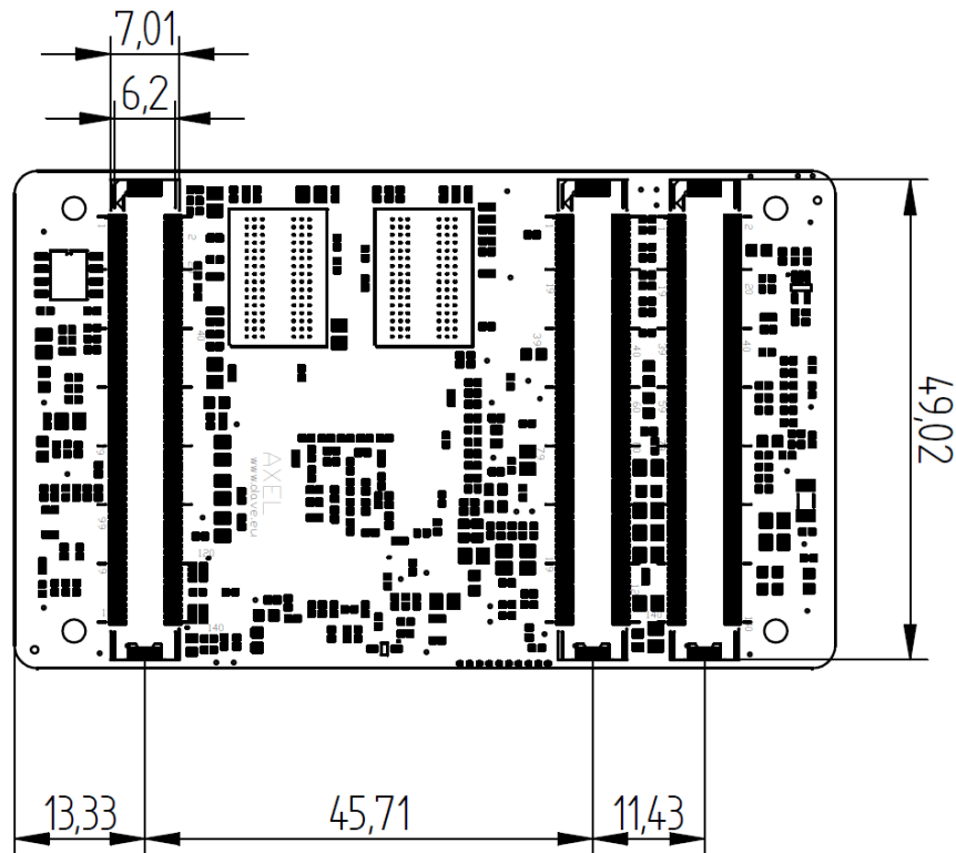
Fig. 5: Connectors layout
