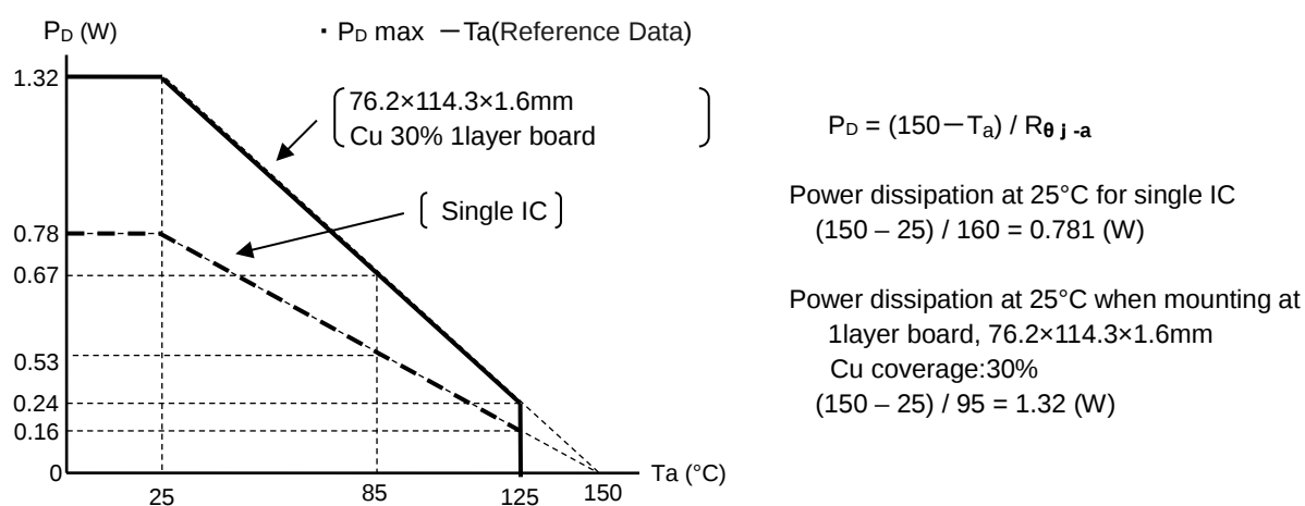
Figure 8.1 Thermal Characteristics
