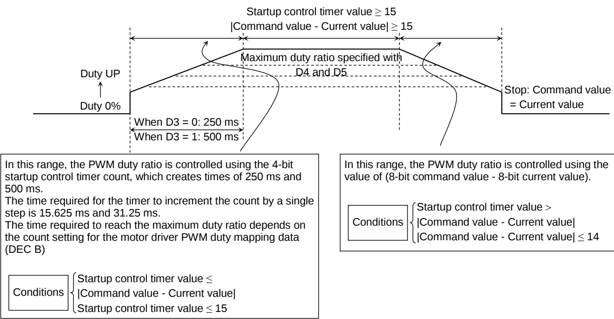
Figure 7.24 PWM Duty Ratio Control
