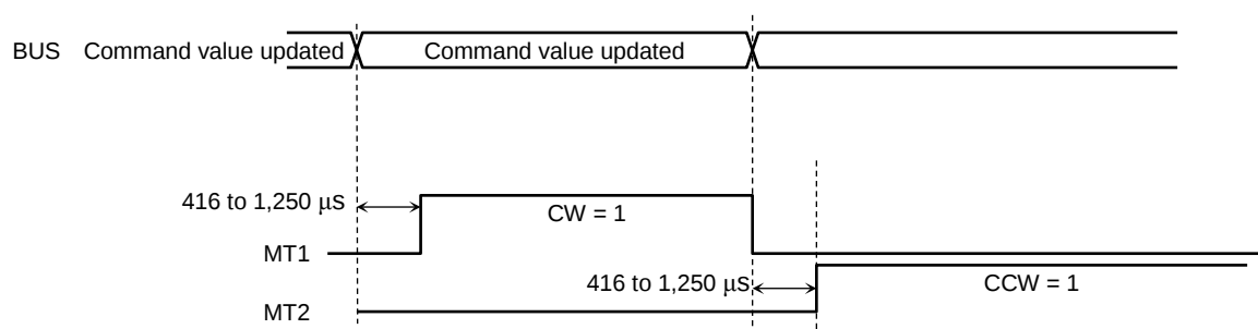
Figure 7.27 Example Motor Driver Operation Timing
