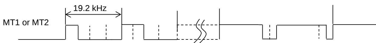
Figure 7.22 PWM signal
