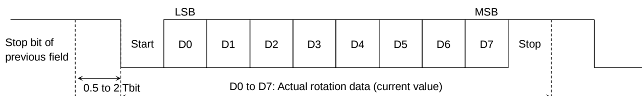
Figure 7.18 DATA1 Field
