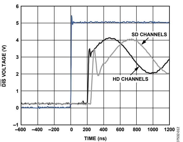
Figure 13. Enable Time
