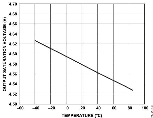
Figure 17. Output Saturation Voltage vs. Temperature
