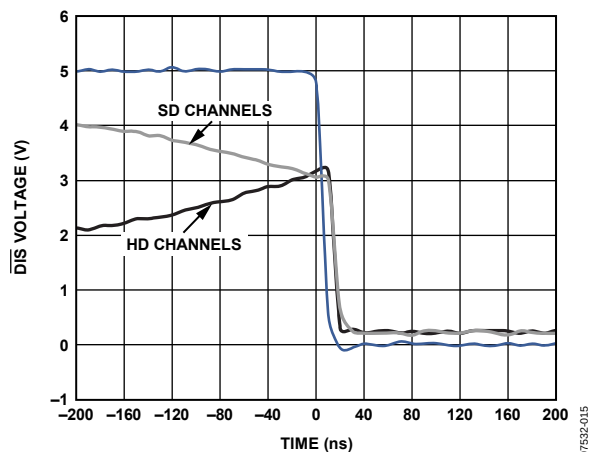
Figure 16. Disable Time
