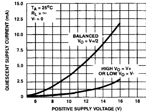
FIGURE 19. QUIESCENT SUPPLY CURRENT vs SUPPLY VOLTAGE
