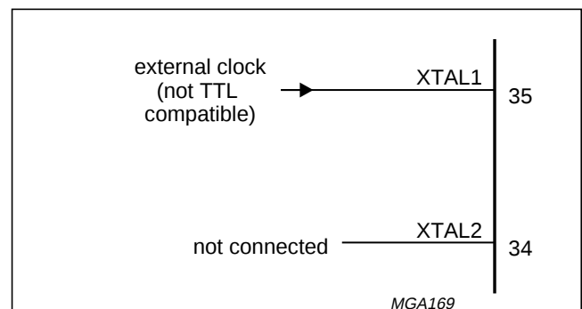
Fig.15 Driving the P8xC562 from an external source.
