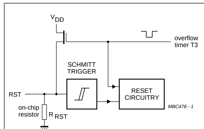
Fig.16 On-chip reset configuration.
