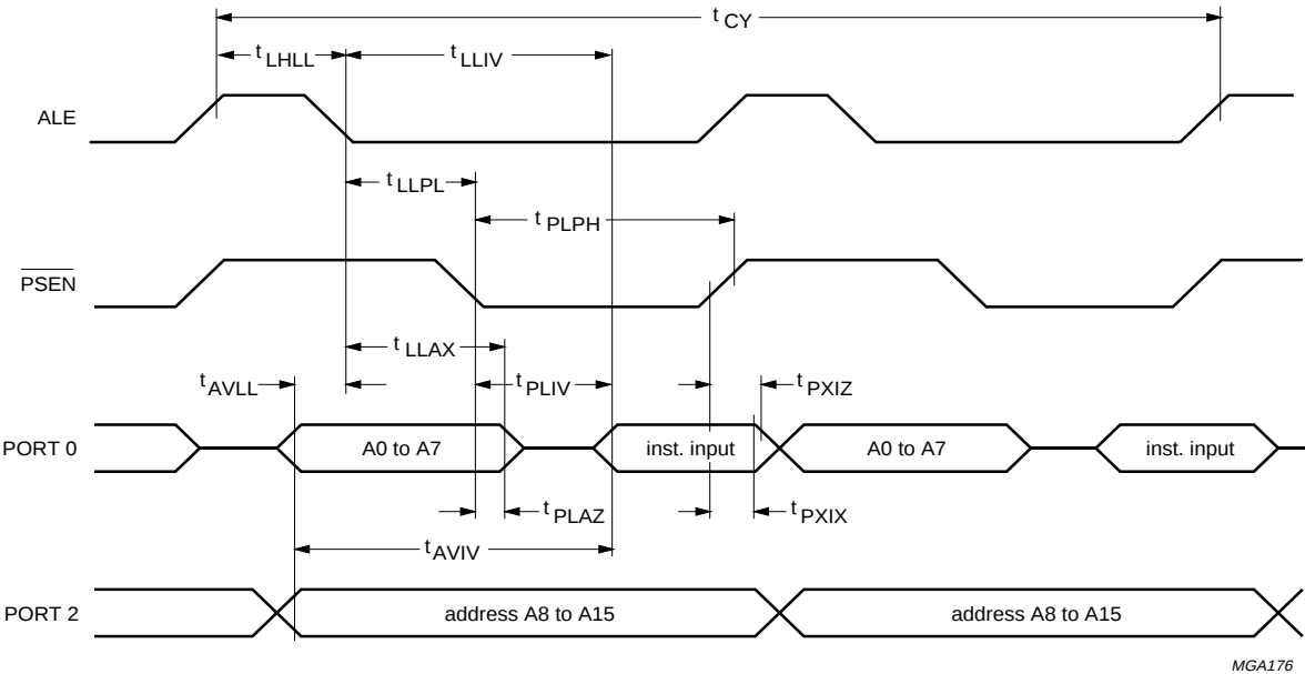
Fig.22 Read from program memory.
