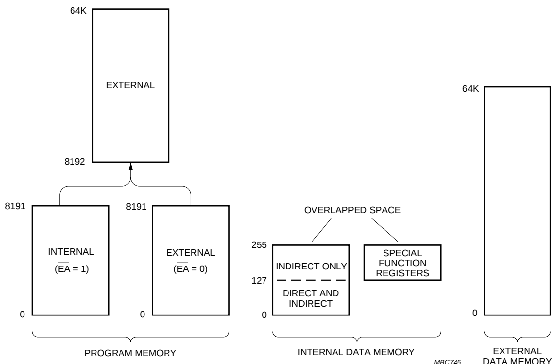
Fig.4 Memory map.
