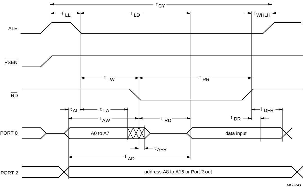
Fig.23 Read from data memory.
