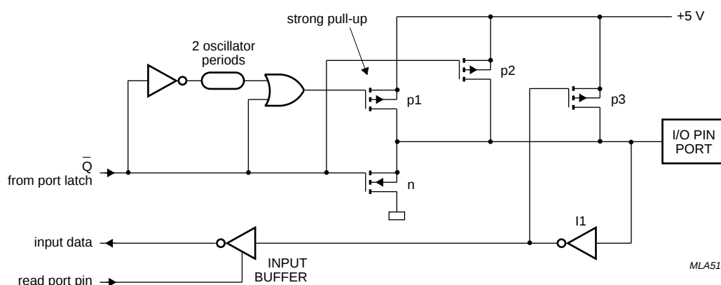
Fig.7 I/O buffers in the P8xC562 (Ports 2, 3, 4 and P1.0 to P1.5).
