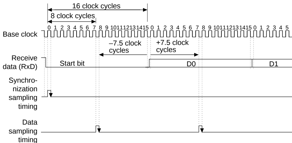
Figure 13.21 Receive Data Sampling Timing in Asynchronous Mode
