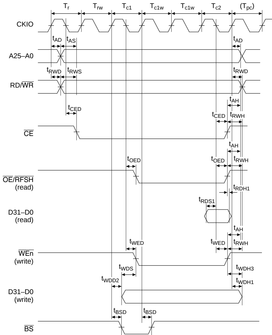
Figure 17.46 Pseudo-SRAM Read Cycle (RCD = 1, A3W = 3, TPC = 0)
