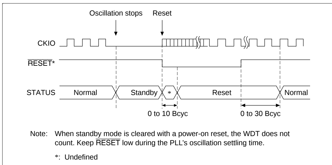
Figure 8.5 Standby to Power-On Reset STATUS Output
