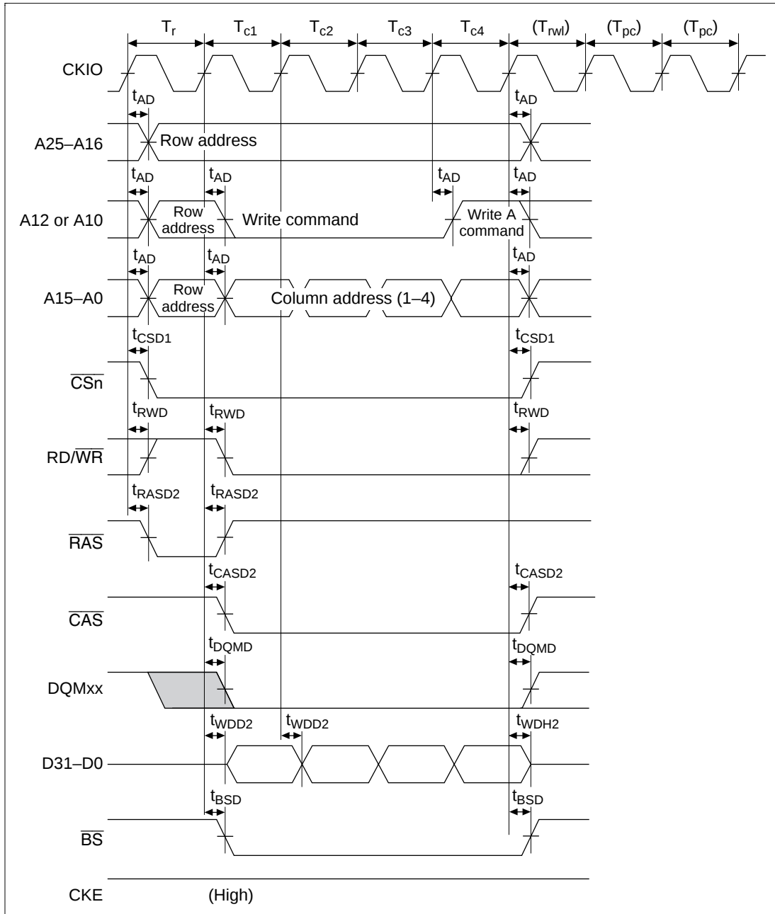
Figure 16.40 Synchronous DRAM Write Bus Cycle (Burst Mode (Single Write x 4), RCD = 0, TPC = 1, TRWL = 0)
