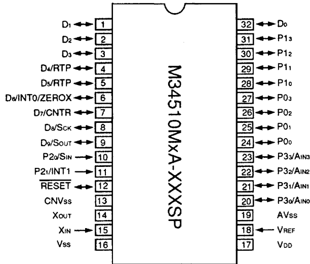
Outline 32P4B
