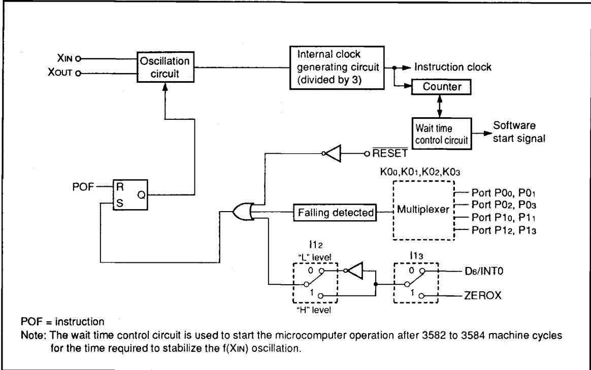
Fig. 44 Clock control circuit structure
