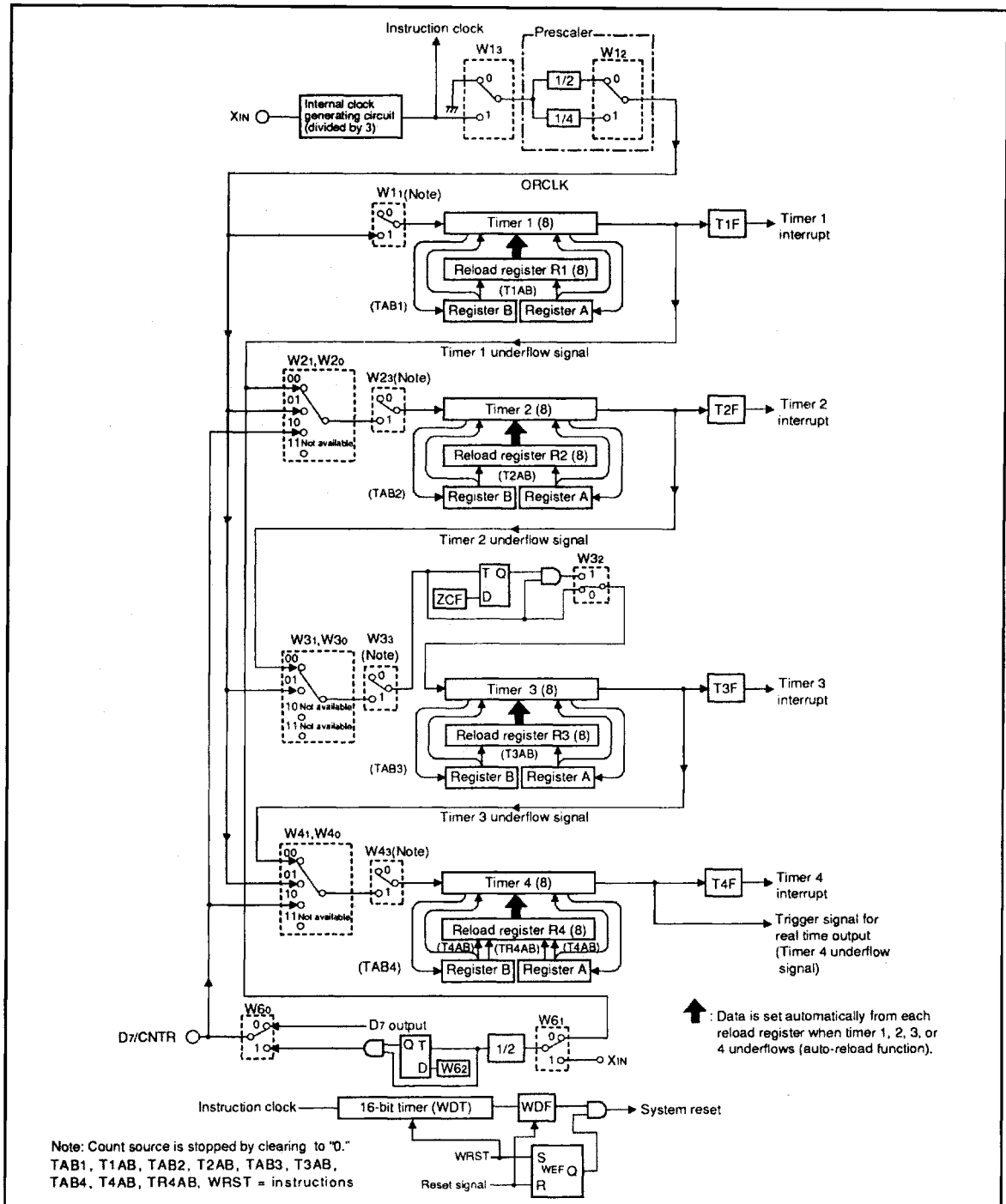
Fig. 21 Timers structure
