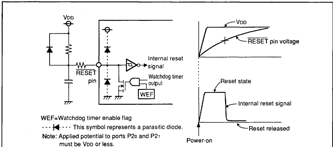
Fig. 37 Power-on reset circuit example
