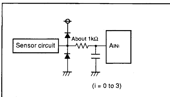
Fig. 51 Analog input external circuit example-2
