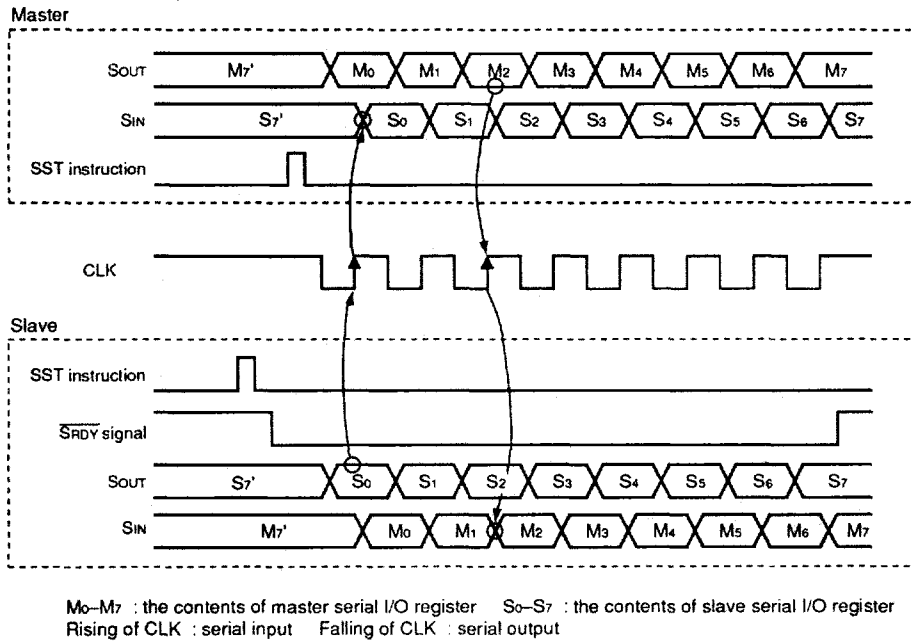
Fig. 30 Timing of serial I/O data transfer
