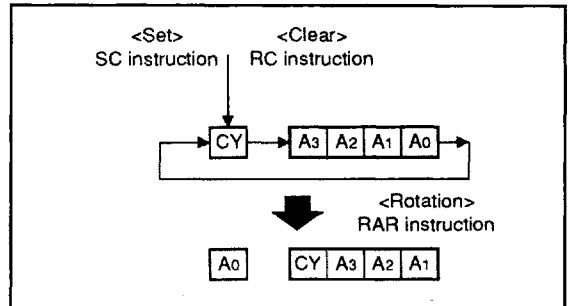
Fig. 2 RAR instruction execution example
