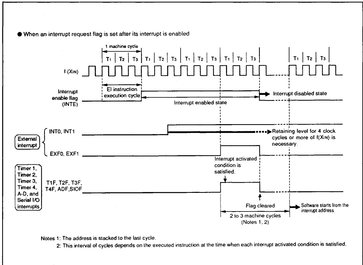
Fig. 16 Interrupt sequence
