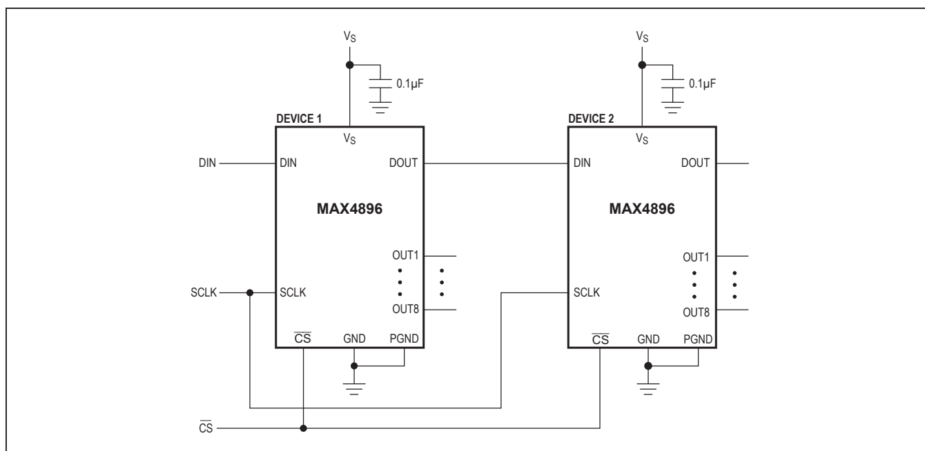
Figure 3. Daisy-Chain Configuration
