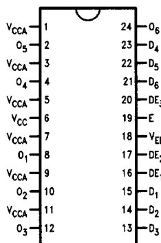
24-Pin DIP
