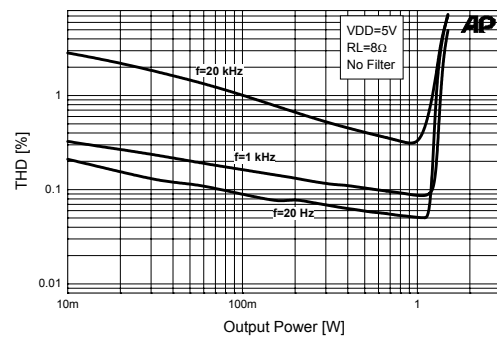
Figure 4. THD+N vs. Output Power, V_{DD} = 5V
