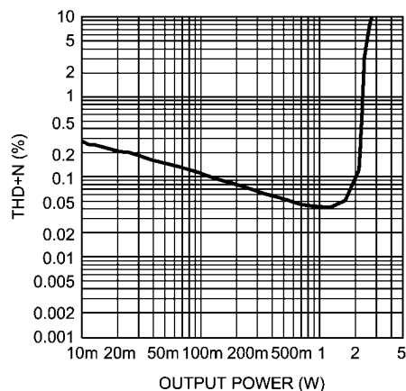
THD+N vs Output Power V_{DD} = 5V , R_L = 15\mu H + 4\Omega + 15\mu H f = 1kHz , Mode 2
