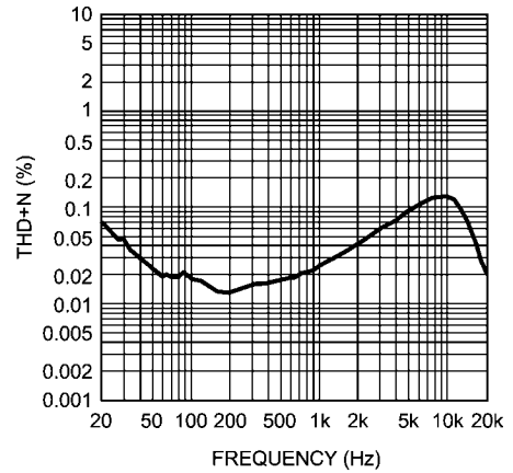
THD+N vs Frequency V_{DD} = 5V , R_L = 5\mu H + 8\Omega + 15\mu H P_{OUT} = 750mW , Mode 2
