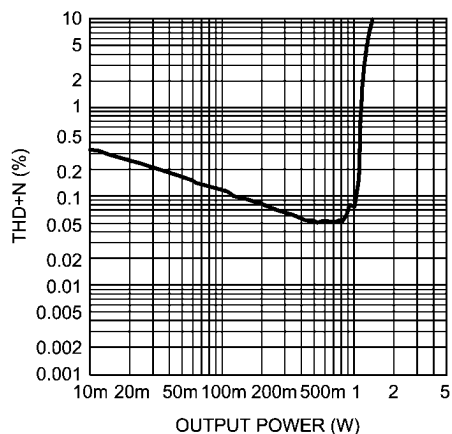
THD+N vs Output Power V_{DD} = 3.6V , R_L = 15\mu H + 4\Omega + 15\mu H f = 1kHz , Mode 3
