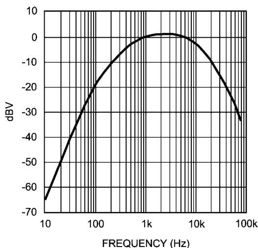
FIGURE 15. A-Weighted Filter
