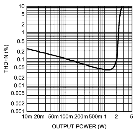
THD+N vs Output Power V_{DD} = 5V , R_L = 15\mu H + 4\Omega + 15\mu H f = 1kHz , Mode 3
