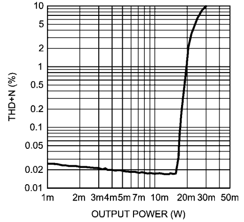
THD+N vs Output Power R_L = 32\Omega , f = 1kHz , Mode 4
