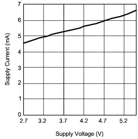
Supply Current vs Supply Voltage Mode 3, Mono Inputs
