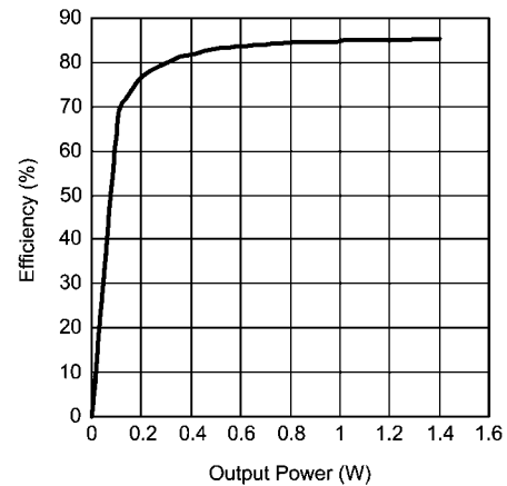
Efficiency vs Output Power R_L = 15\mu\text{H} + 4\Omega + 15\mu\text{H} , f = 1\text{kHz} , V_{DD} = 3.6\text{V}
