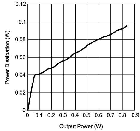
Power Dissipation vs Output Power R_L = 15\mu\text{H} + 8\Omega + 15\mu\text{H} , f = 1\text{kHz} , V_{DD} = 3.6\text{V}
