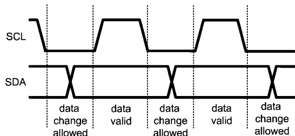
FIGURE 3. I 2 C Signals: Data Validity
