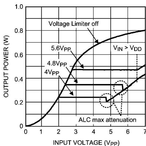
FIGURE 13. Voltage Limiter Function V_{DD} = 3.3V , R_L = 15\mu H + 8\Omega + 15\mu H f_{IN} = 1kHz , LS_GAIN = 0
