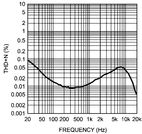
THD+N vs Frequency V_{DD} = 5V , R_L = 15\mu H + 8\Omega + 15\mu H P_{OUT} = 50mW , Mode 3
