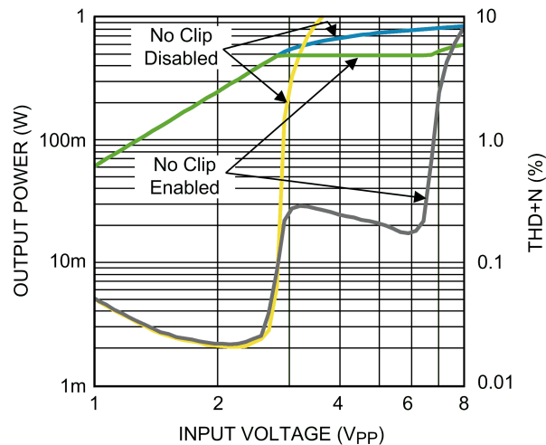
FIGURE 14. No Clip Function V_{DD} = 3.3V , R_L = 15\mu H + 8\Omega + 15\mu H f_{IN} = 1kHz , LS\_GAIN = 0 Blue, Green = Output Power vs Input Voltage Gray, Yellow = THD+N vs Input Voltage
