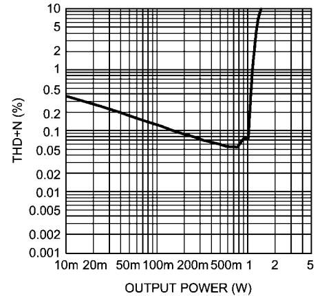
THD+N vs Output Power V_{DD} = 3.6V , R_L = 15\mu H + 4\Omega + 15\mu H f = 1kHz , Mode 2
