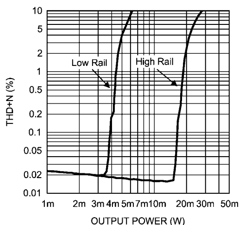
FIGURE 9. Class G Disabled (Low/High Supply Rails)
