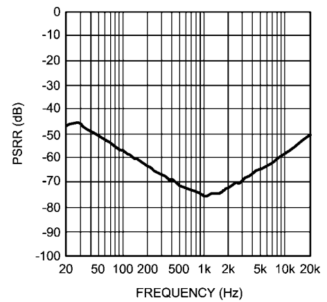
PSRR vs Frequency R_L = 15\mu\text{H}+8\Omega+15\mu\text{H} , f = 1\text{kHz} , V_{DD} = 3.6\text{V} A_V = 6\text{dB} , Mode 2
