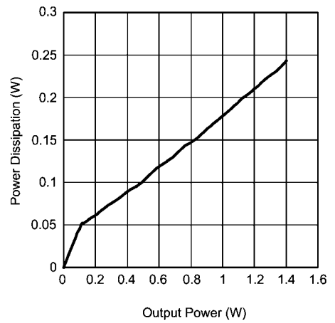
Power Dissipation vs Output Power R_L = 15\mu H + 4\Omega + 15\mu H , f = 1kHz , V_{DD} = 3.6V
