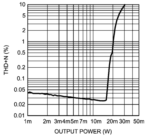
THD+N vs Output Power R_L = 16\Omega , f = 1kHz , Mode 4
