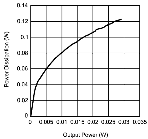
Power Dissipation vs Output Power R_L = 16\Omega , f = 1\text{kHz} , V_{DD} = 1.8\text{V}
