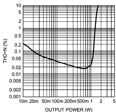
THD+N vs Output Power V_{DD} = 5V , R_L = 15\mu H + 8\Omega + 15\mu H f = 1kHz , Mode 2
