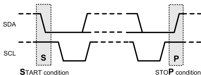
FIGURE 4. I 2 C Start and Stop Conditions
