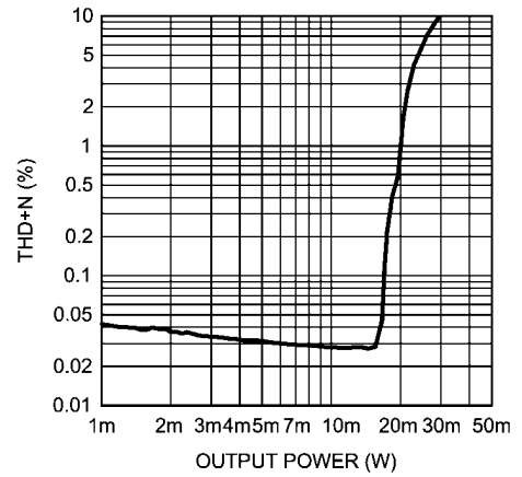
THD+N vs Output Power R_L = 16\Omega , f = 1kHz , Mode 6
