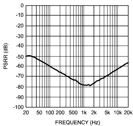
PSRR vs Frequency R_L = 15\mu\text{H}+8\Omega+15\mu\text{H} , V_{DD} = 5\text{V} A_V = 6\text{dB} , Mode 2
