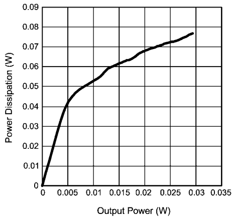
Power Dissipation vs Output Power R_L = 32\Omega , f = 1\text{kHz} , V_{DD} = 1.8\text{V}
