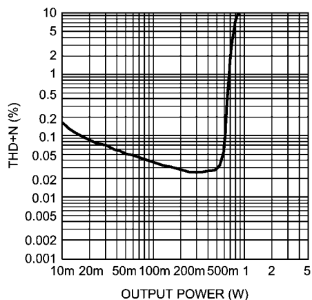
THD+N vs Output Power V_{DD} = 3.6V , R_L = 15\mu H + 8\Omega + 15\mu H f = 1kHz , Mode 2
