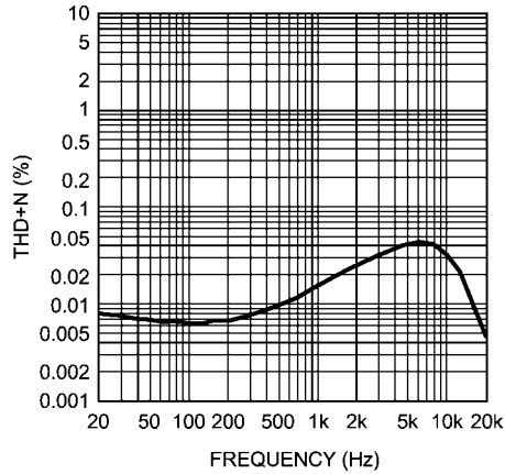
THD+N vs Frequency R_L = 32\Omega P_{OUT} = 14mW , Mode 4
