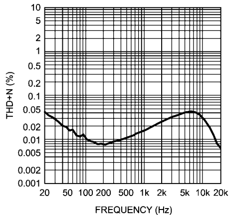
THD+N vs Frequency R_L = 32\Omega P_{OUT} = 14mW , Mode 6
