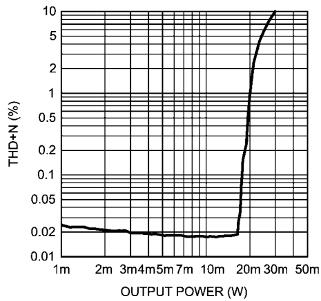
THD+N vs Output Power R_L = 32\Omega , f = 1kHz , Mode 6
