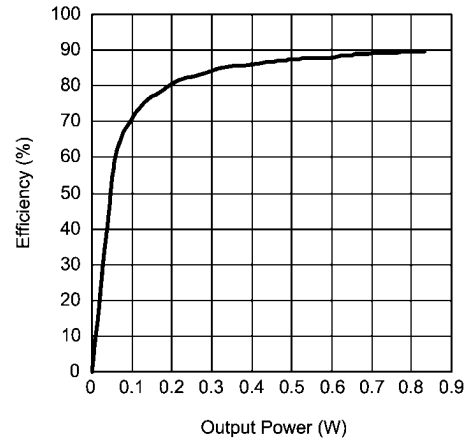
Efficiency vs Output Power R_L = 15\mu\text{H}+8\Omega+15\mu\text{H} , f = 1\text{kHz} , V_{DD} = 3.6\text{V}
