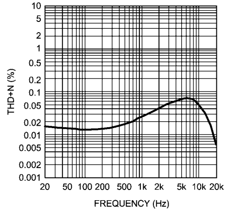
THD+N vs Frequency R_L = 16\Omega P_{OUT} = 14mW , Mode 4
