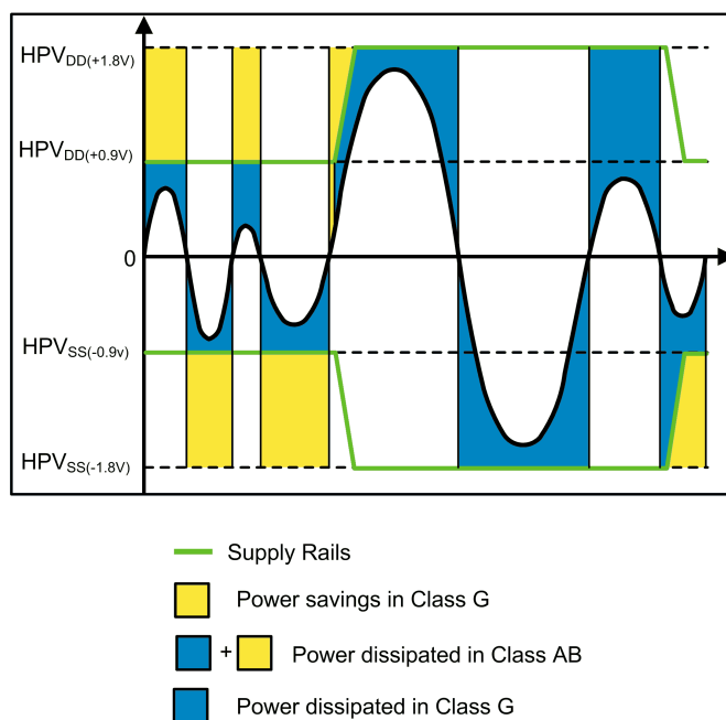
FIGURE 8. Class G Operation
