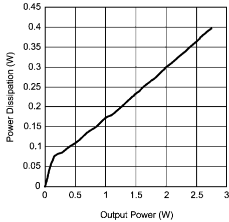
Power Dissipation vs Output Power R_L = 15\mu\text{H} + 4\Omega + 15\mu\text{H} , f = 1\text{kHz} , V_{DD} = 5\text{V}
