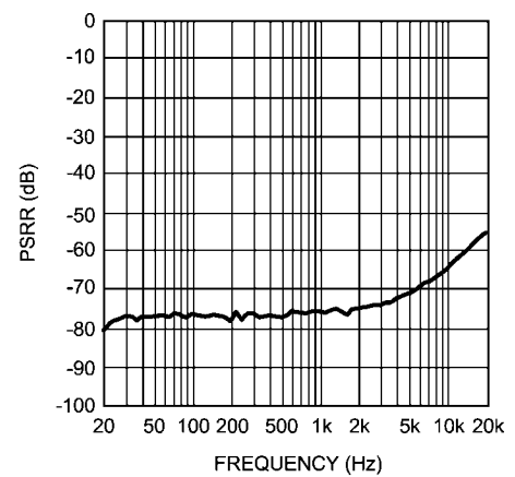
PSRR vs Frequency R_L = 15\mu\text{H}+8\Omega+15\mu\text{H} , V_{DD} = 3.6\text{V} A_V = 6\text{dB} , Mode 3
