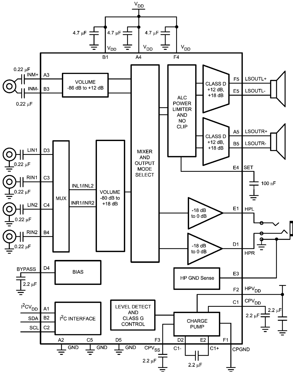
FIGURE 2. Typical Audio Amplifier Application Circuit
