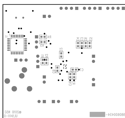
Bottom Silkscreen
