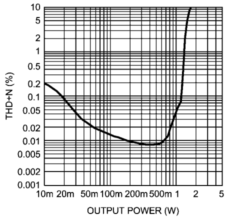
THD+N vs Output Power V_{DD} = 5V , R_L = 15\mu H + 8\Omega + 15\mu H f = 1kHz , Mode 3
