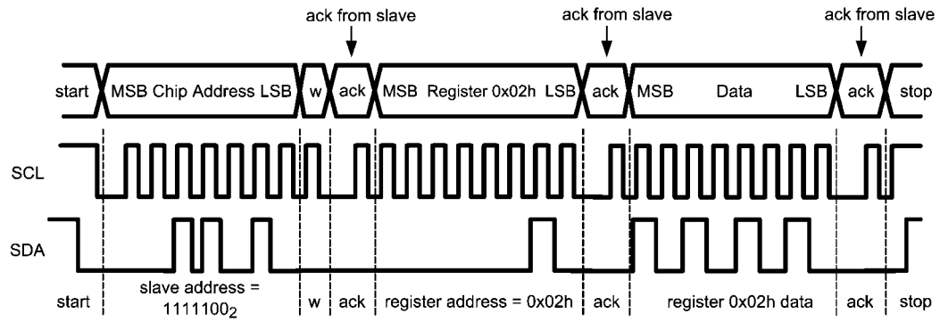
FIGURE 6. Example I²C Write Cycle
