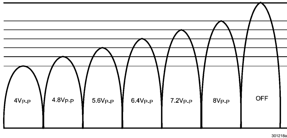
FIGURE 10. Voltage Limit Output Level
