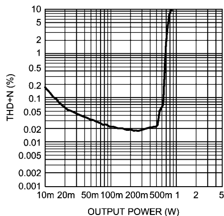
THD+N vs Output Power V_{DD} = 3.6V , R_L = 15\mu H + 8\Omega + 15\mu H f = 1kHz , Mode 3
