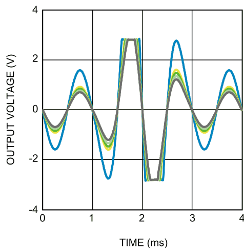
FIGURE 12. Clip Control Levels V_{DD} = 3.3V , V_{IN} = 8V_{PP} Shaped Burst, 1kHz Blue = No Clip Disabled, Gray = Low, Light Green = Medium Green = High, Yellow = Max
