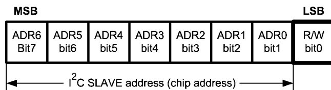
FIGURE 5. I 2 C Chip Address
