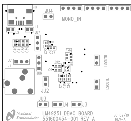
Top Silkscreen
