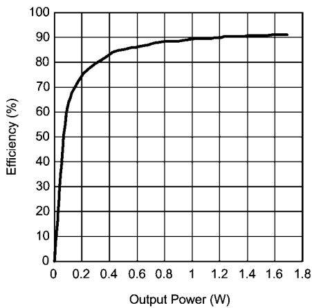
Efficiency vs Output Power R_L = 15\mu\text{H}+8\Omega+15\mu\text{H} , f = 1\text{kHz} , V_{DD} = 5\text{V}
