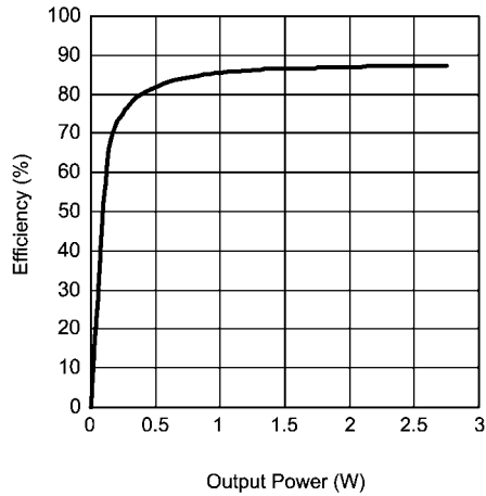
Efficiency vs Output Power R_L = 15\mu\text{H}+4\Omega+15\mu\text{H} , f = 1\text{kHz} , V_{DD} = 5\text{V}
