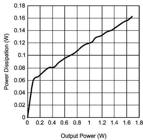
Power Dissipation vs Output Power R_L = 15\mu\text{H} + 8\Omega + 15\mu\text{H} , f = 1\text{kHz} , V_{DD} = 5\text{V}
