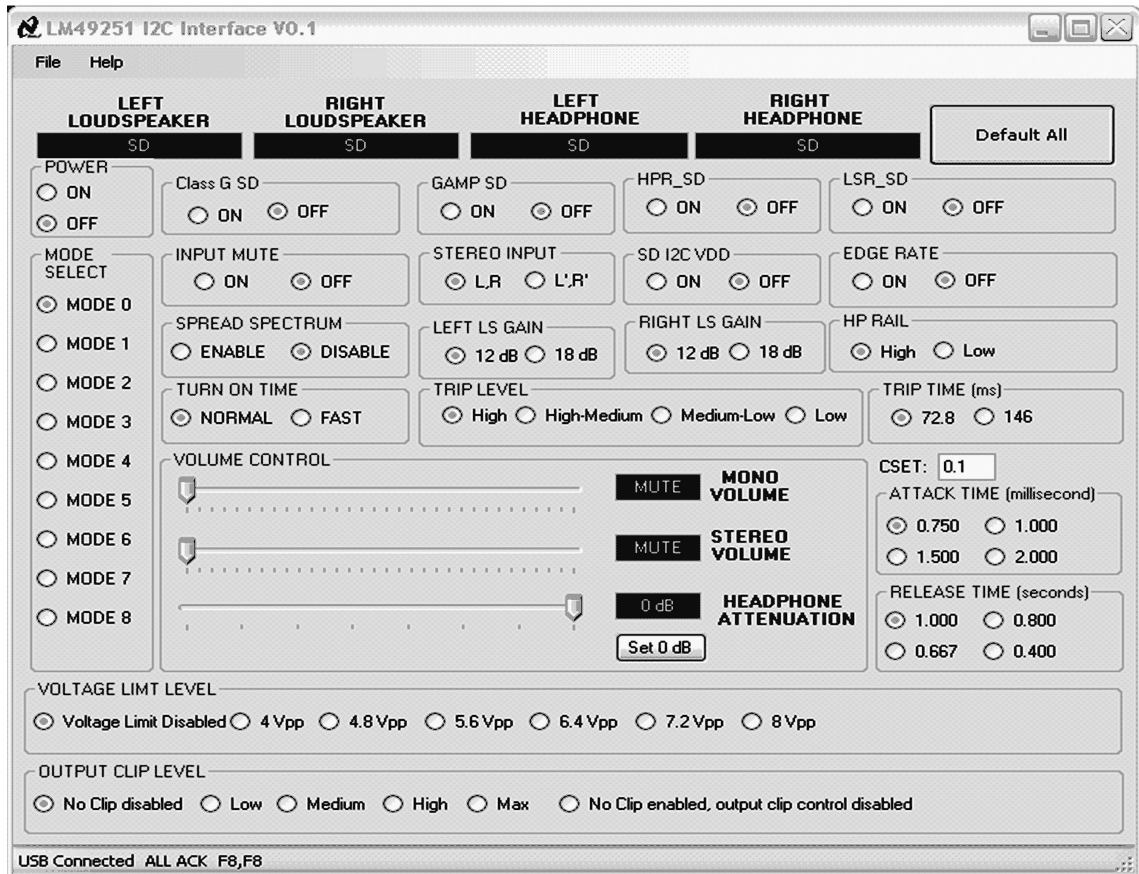
FIGURE 16. Software Graphic user Interface (GUI)
