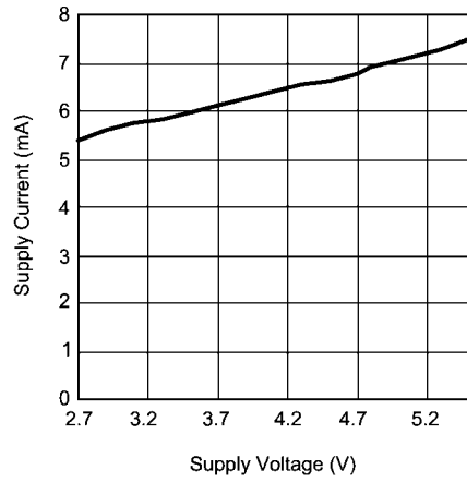
Supply Current vs Supply Voltage Mode 8, Stereo Inputs
