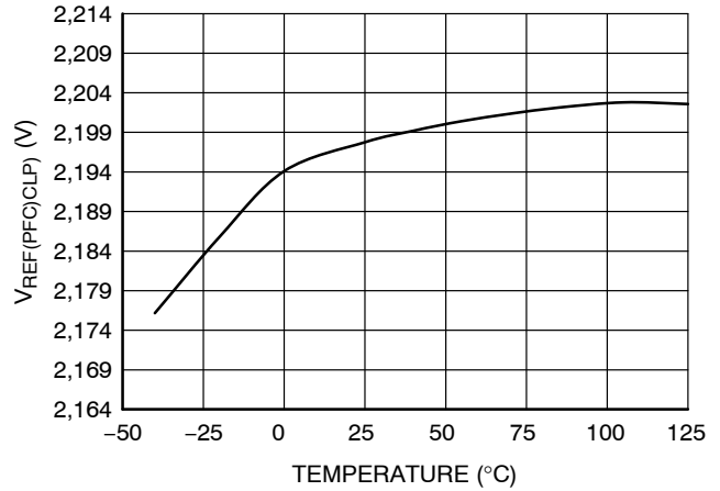
Figure 12. V_{REF(PFC)CLP} vs. Temperature
