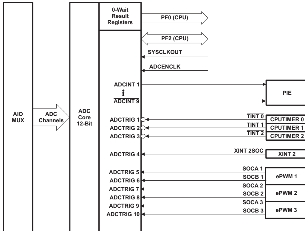
Figure 6-3. ADC Connections
