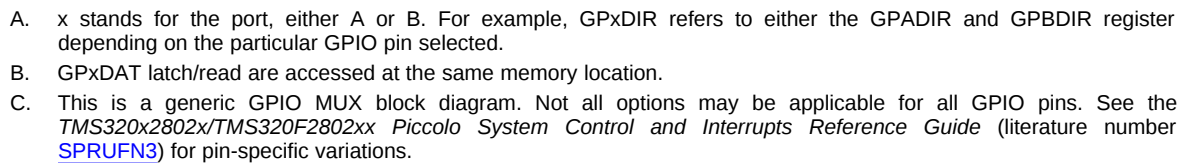
Figure 6-27. GPIO Multiplexing
