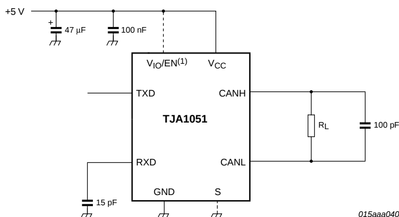
Fig 7. Timing test circuit for CAN transceiver
