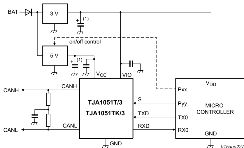
Fig 6. Typical application of the TJA1051T/3 or TJA1051TK/3.
