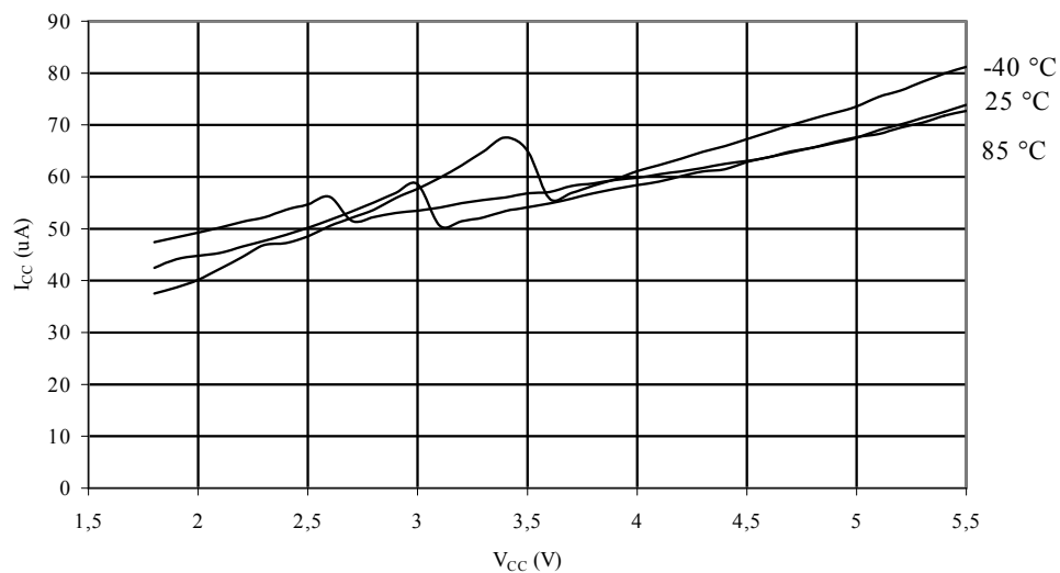
Figure 30-43. AREF External Reference Current vs. V_{CC}
