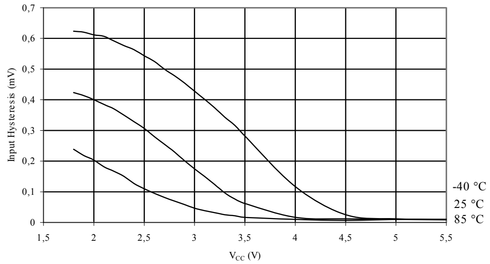
Figure 30-30. Reset Pin Input Hysteresis vs. V_{CC}
