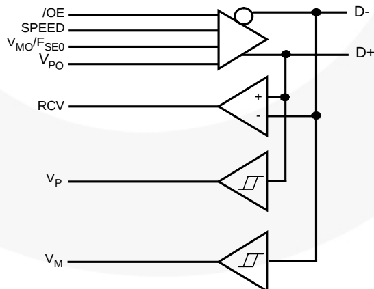
Figure 1. Logic Diagram
