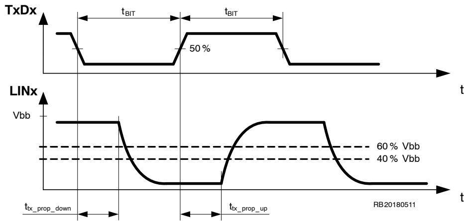
Figure 7. LIN Transmitter Timing
