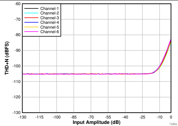
Figure 5. THD+N vs Input Amplitude
