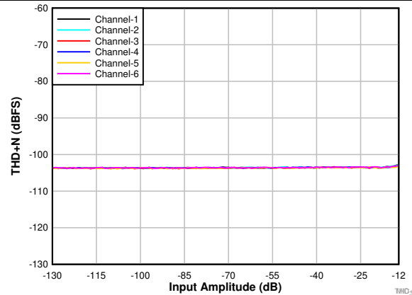
DC-coupled single-ended microphone input with DC common-mode 1N \times P = 4\text{ V} and IN \times M = 0\text{ V} , high swing mode enabled
