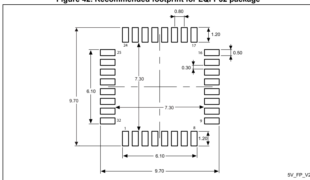
Figure 42. Recommended footprint for LQFP32 package
