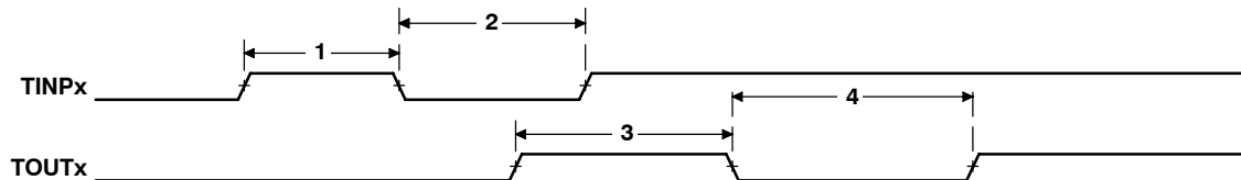
Figure 55. Timer Timing
