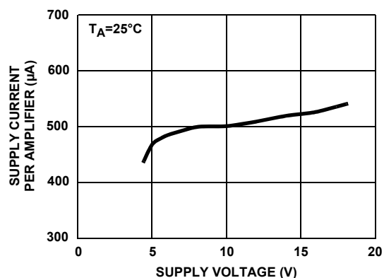
FIGURE 10. SUPPLY CURRENT PER AMPLIFIER vs SUPPLY VOLTAGE
