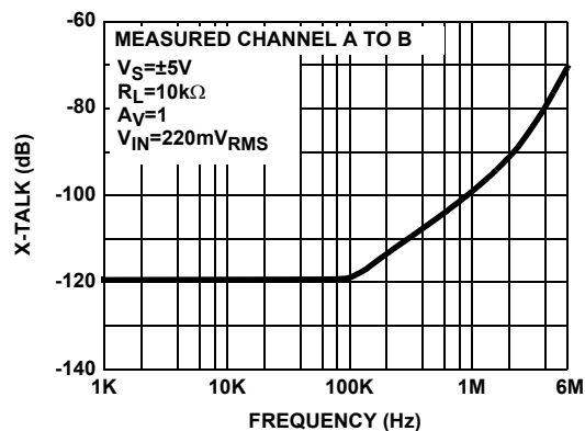
FIGURE 20. CHANNEL SEPARATION vs FREQUENCY RESPONSE
