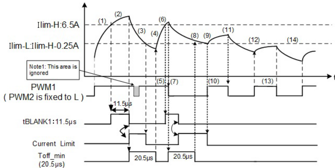
Figure 7.14 Chopper-type current-limit control
