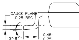
DETAIL "A"
