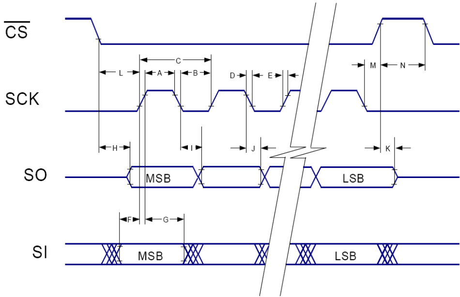
Figure 8. SPI Timing
