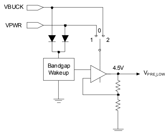
Figure 32. V_{PRE\_LOW} Regulator
