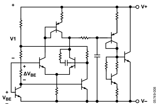
Figure 7. Schematic Diagram
