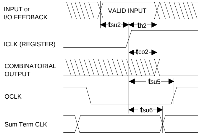
Registered Input
