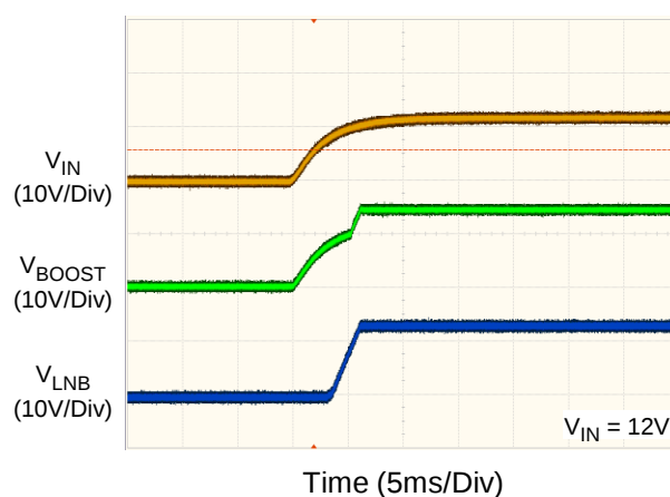
Power On Sequence
