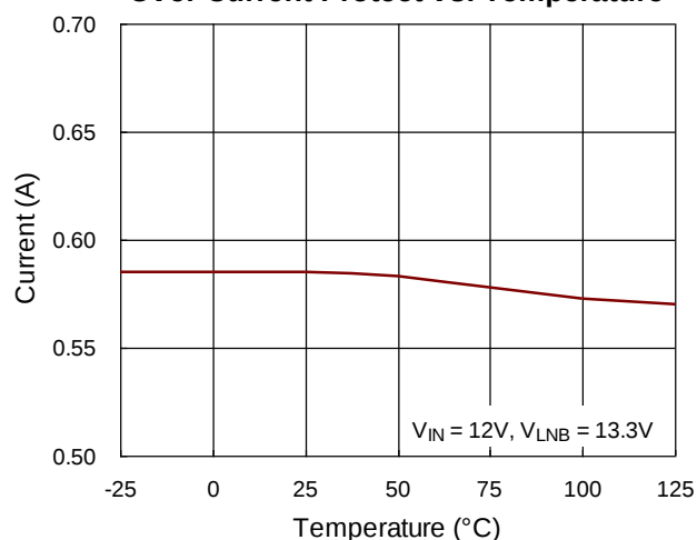
Over Current Protect vs. Temperature
