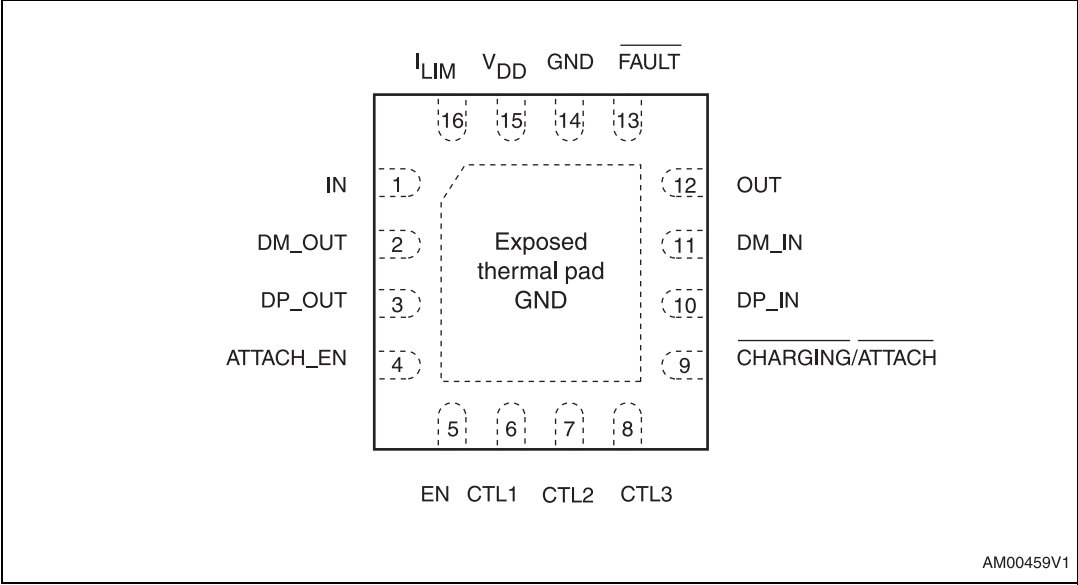
Figure 2. Pinout
