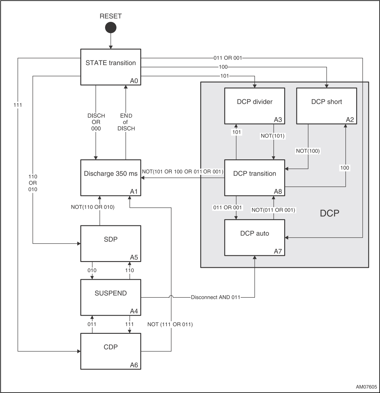
Figure 5. State machine
