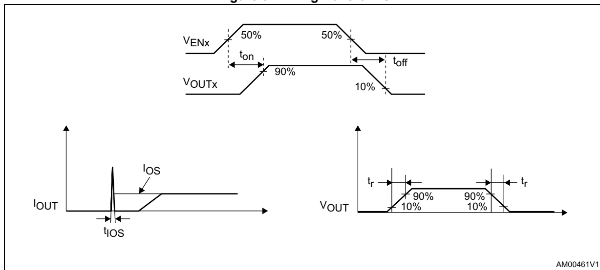
Figure 3. Timing waveforms
