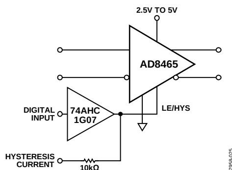
Figure 25. Hysteresis Adjustment with Latch
