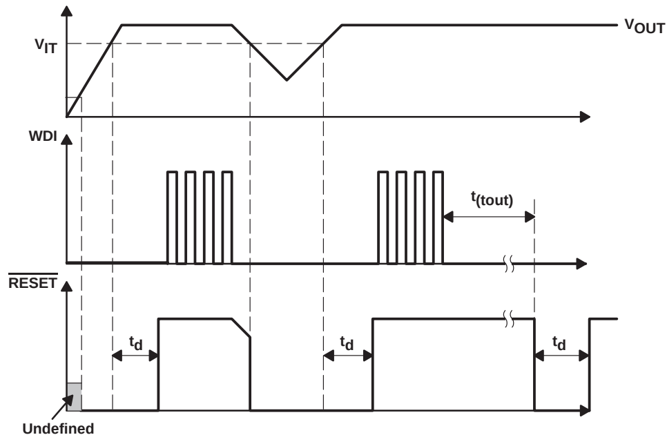
Figure 4. Watchdog Timing
