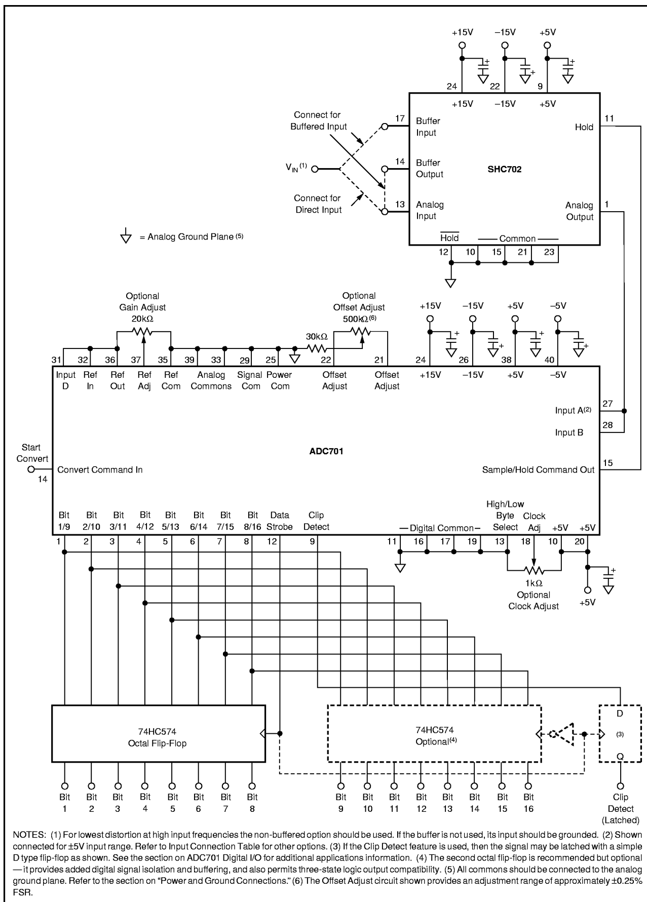
FIGURE 3. ADC701/SHC702 Connection Diagram.
