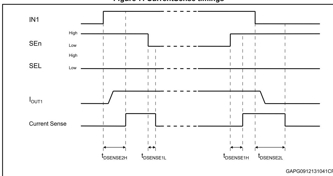
Figure 7: CurrentSense timings
