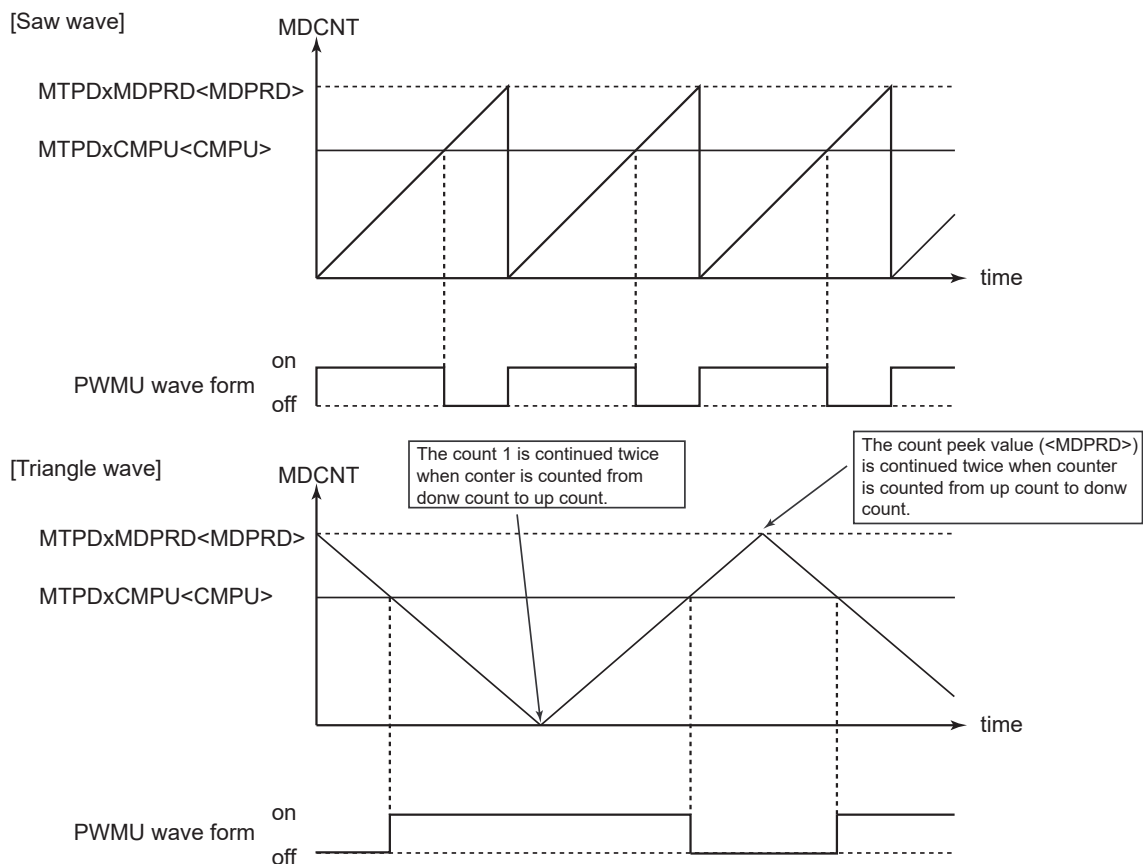
Figure 24-23 PWM waveform
