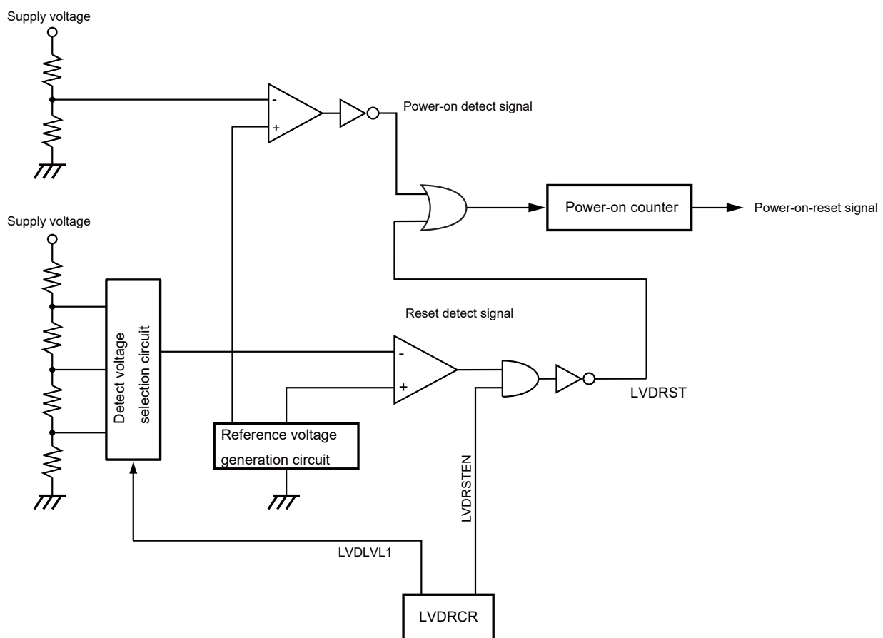
Figure 27-1 Power-on-reset circuit
