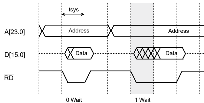
Figure 10-3 Read Operation Timing (0 Wait and 1 Wait Automatically Inserted)
