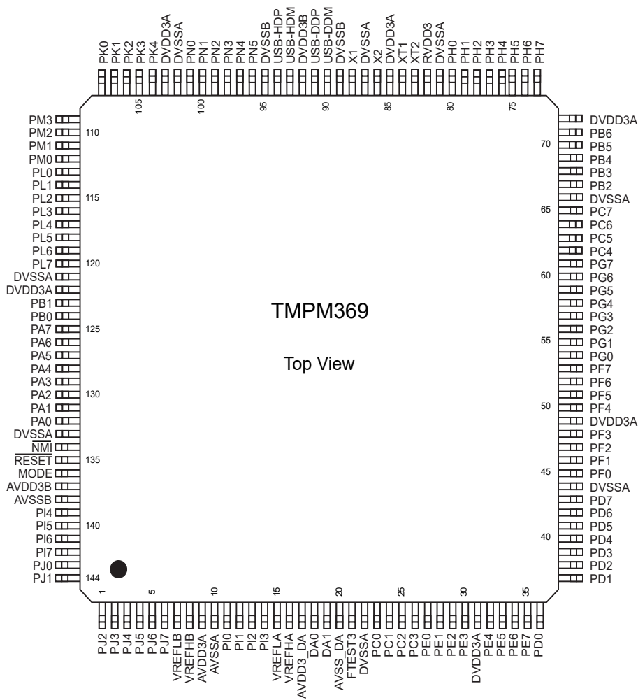
Figure 1-2 Pin Layout
