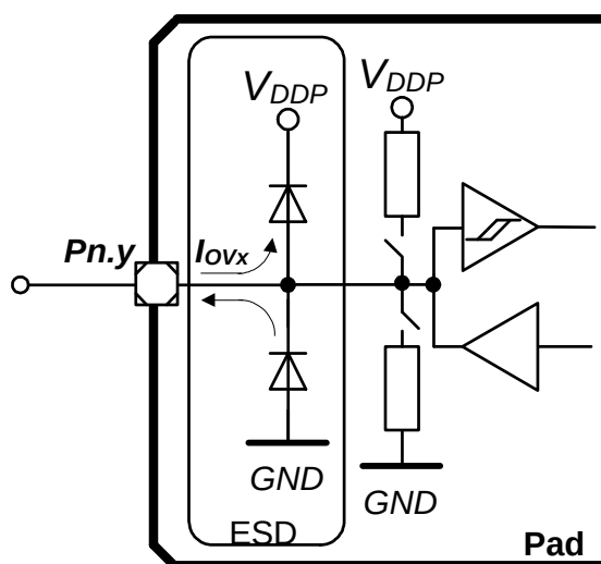
Figure 10 Input Overload Current via ESD structures
