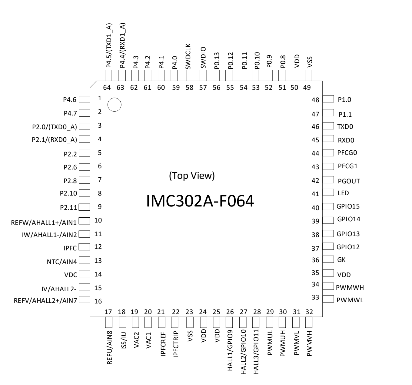
Figure 5 IMC302A-F064
