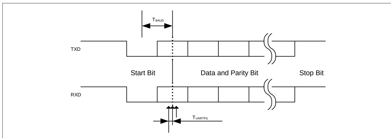
Figure 10 UART timing
