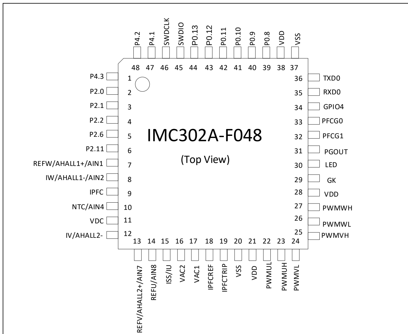
Figure 4 IMC302A-F048
