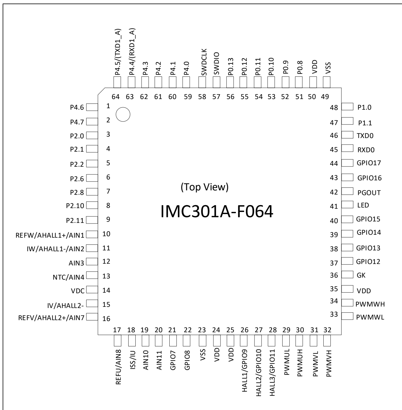
Figure 3 IMC301A-F064
