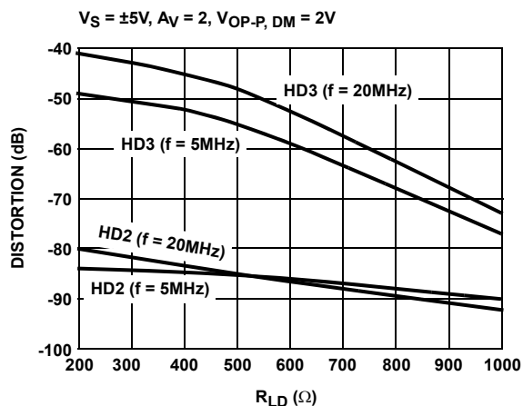
FIGURE 18. HARMONIC DISTORTION vs R_{LD}
