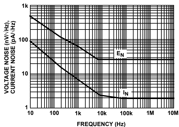
FIGURE 13. VOLTAGE AND CURRENT NOISE vs FREQUENCY
