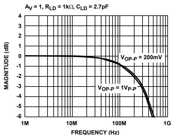
FIGURE 3. FREQUENCY RESPONSE
