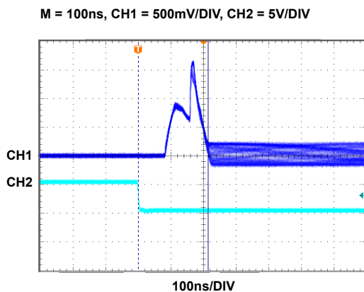
FIGURE 22. ENABLED RESPONSE
