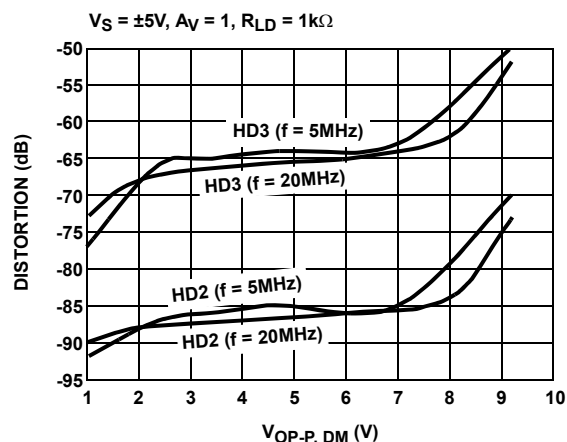
FIGURE 16. HARMONIC DISTORTION vs DIFFERENTIAL OUTPUT VOLTAGE
