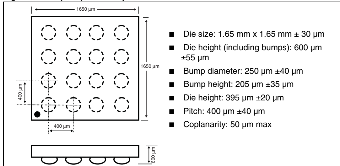
Figure 78. Flip-chip - 16 bumps
