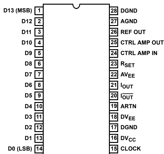
HI5741 (PDIP, SOIC) TOP VIEW
