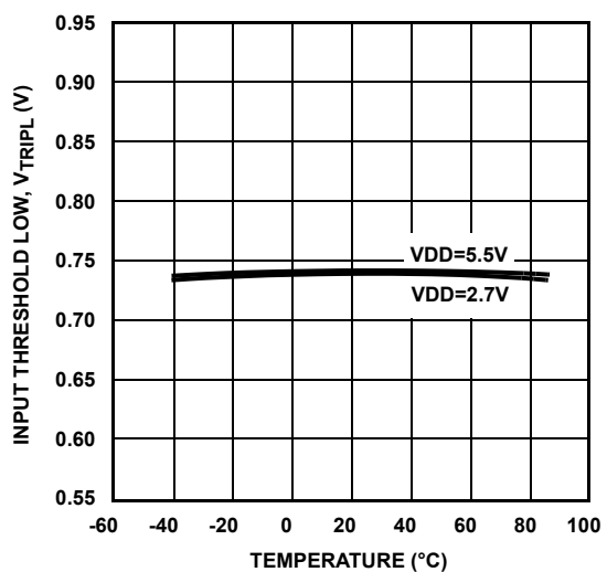
FIGURE 4. V_{TRIPL} VOLTAGE
