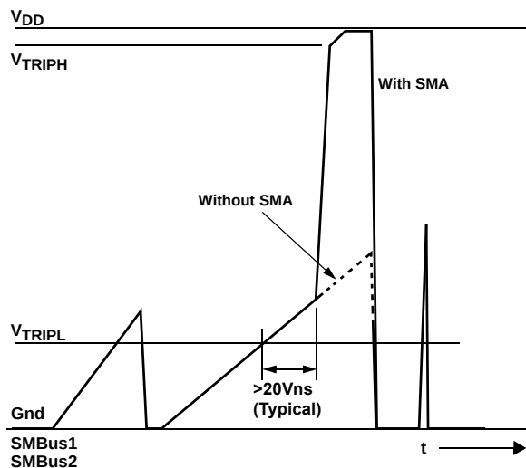
FIGURE 10. NOISE SUPPRESSION. BOOST CURRENT APPLIED WHEN INPUT SIGNAL EXCEEDS 20V_{ns} (TYPICAL).
