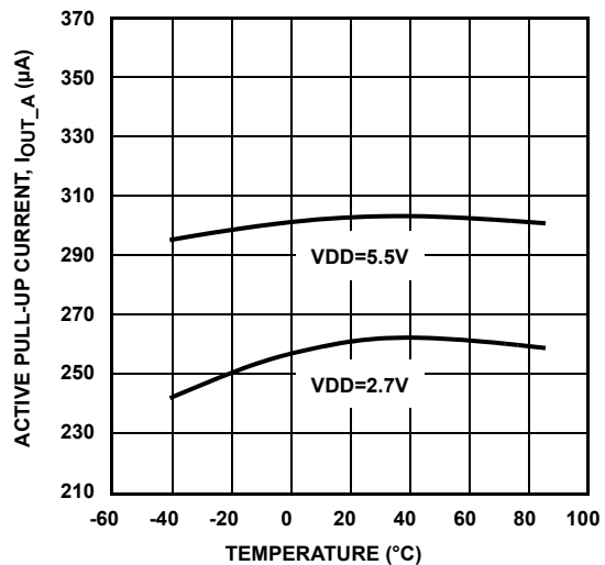
FIGURE 1. ACTIVE PULL-UP CURRENT. SMBus PIN=0V
