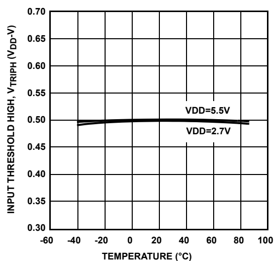
FIGURE 5. V_{TRIPH} VOLTAGE
