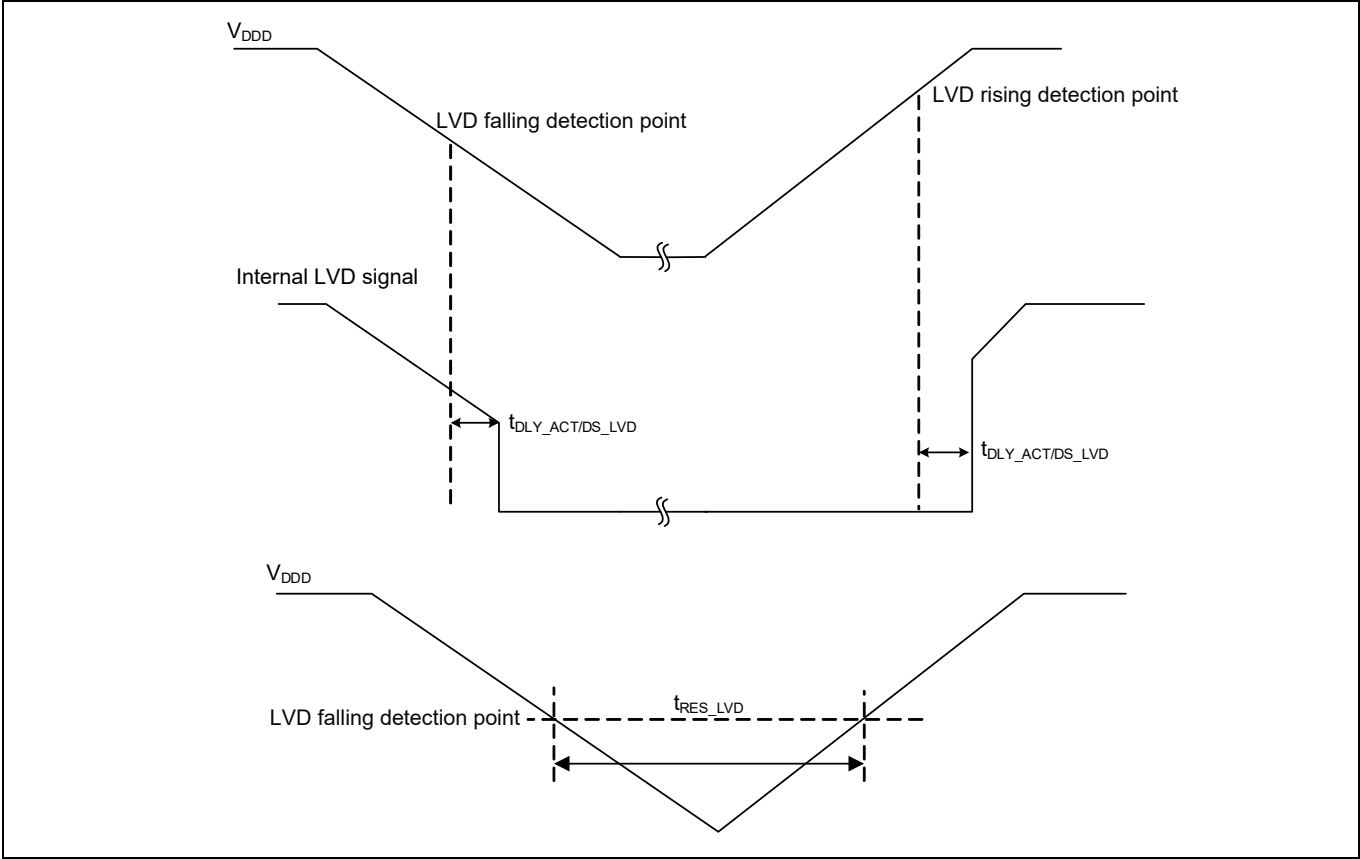
Figure 27-21 LVD specifications
