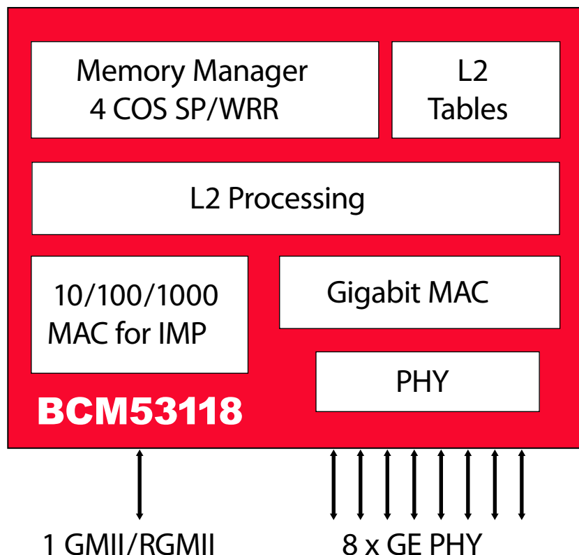
BCM53118 Block Diagram
