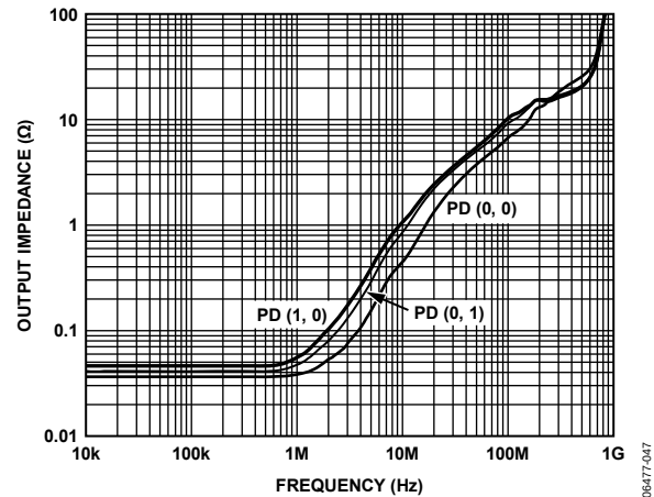
Figure 13. Output Impedance vs. Frequency V_S = \pm 12 V, G = +5 , R_F = 2 k \Omega
