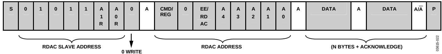
Figure 22. RDAC Write
