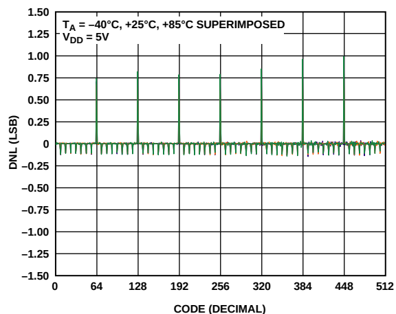
Figure 5. DNL—9-Bit RDAC
