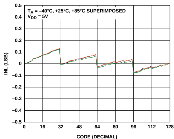
Figure 8. INL—7-Bit RDAC
