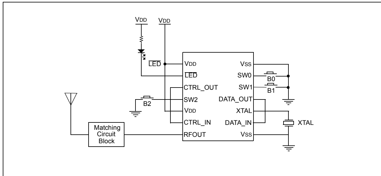
FIGURE 2-1: TYPICAL CIRCUIT
